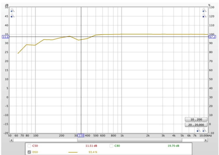
Speech Intelligibility
