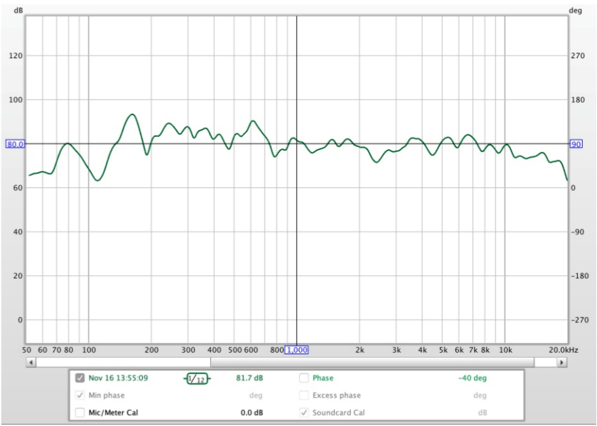
Frequency Response
