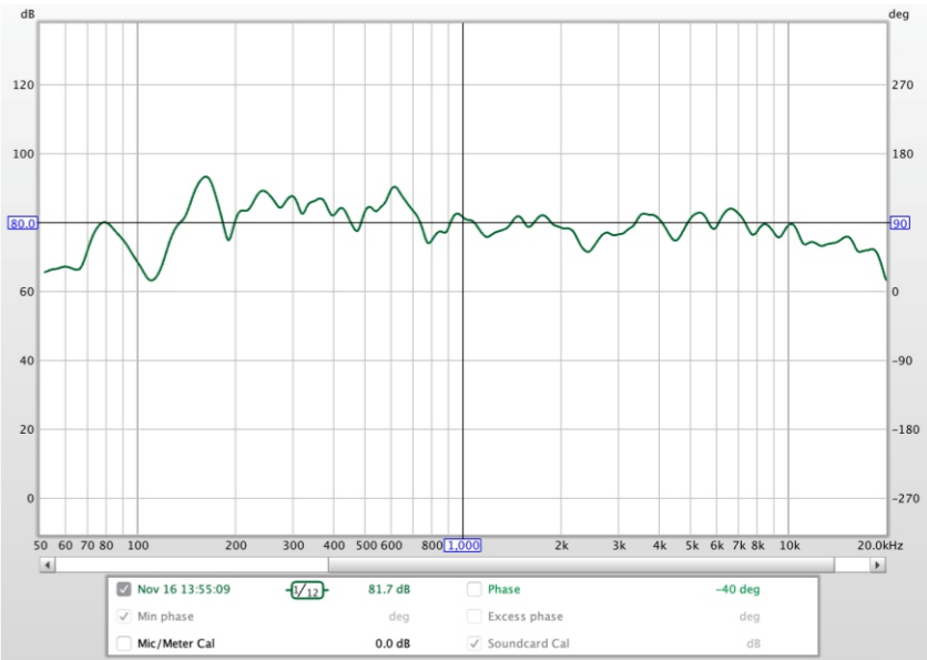
Technical Chart for Office Pod, 1 - 2 Person
