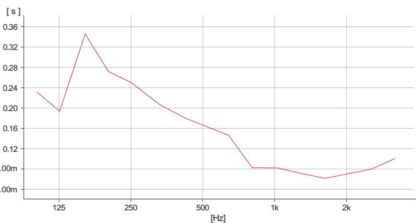
Reverberation Time Test
