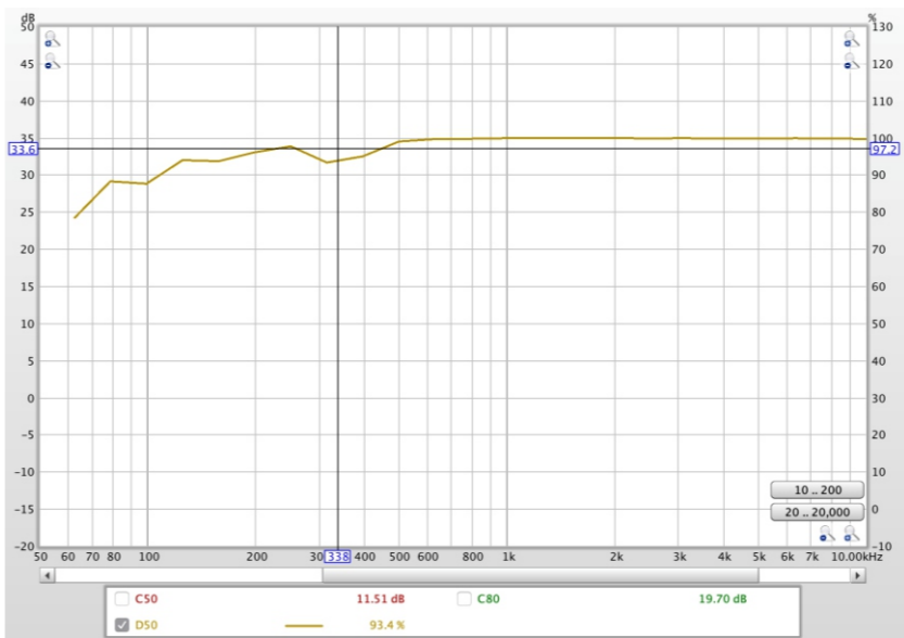
Speech Intelligibility
