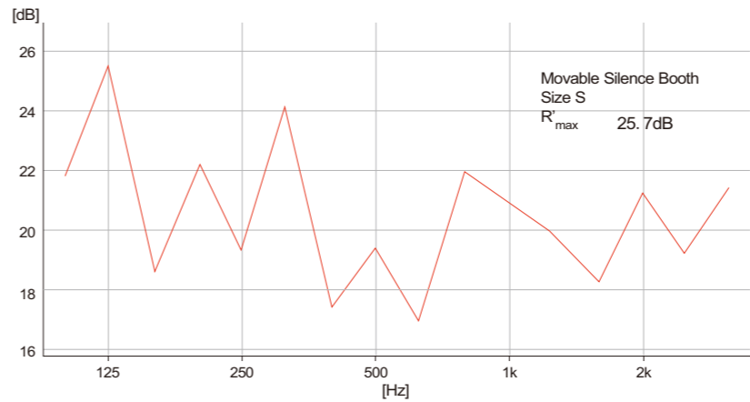
Sound Insulation Test
